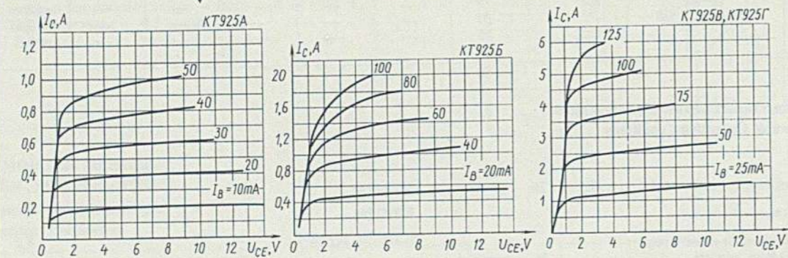
Standard output characteristics for common-emitter circuit
