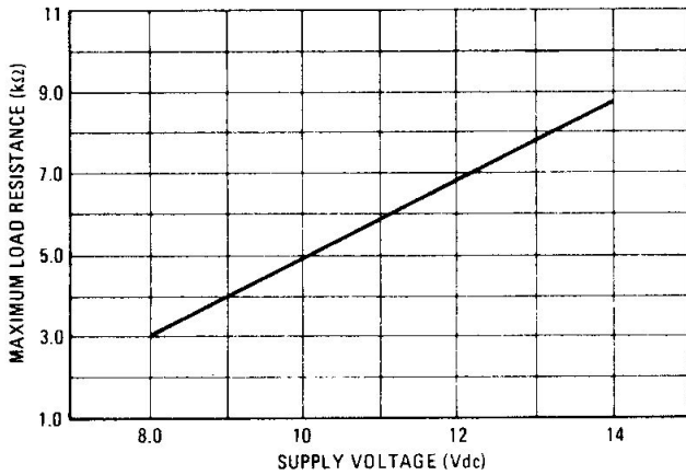
FIGURE 17 – MAXIMUM LOAD RESISTANCE versus SUPPLY VOLTAGE
