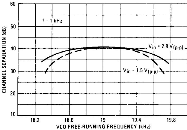
FIGURE 5 – CHANNEL SEPARATION versus VCO FREE-RUNNING FREQUENCY
